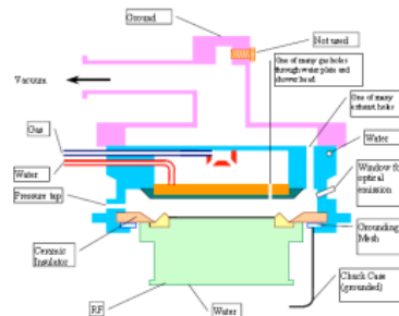
Production-proven Reactor
